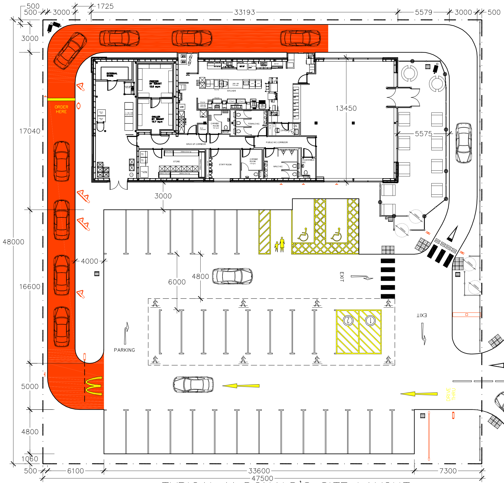
TYPICAL McDONALD'S SITE LAYOUT INCORPORATING AN F85 BUILDING FOOTPRINT
