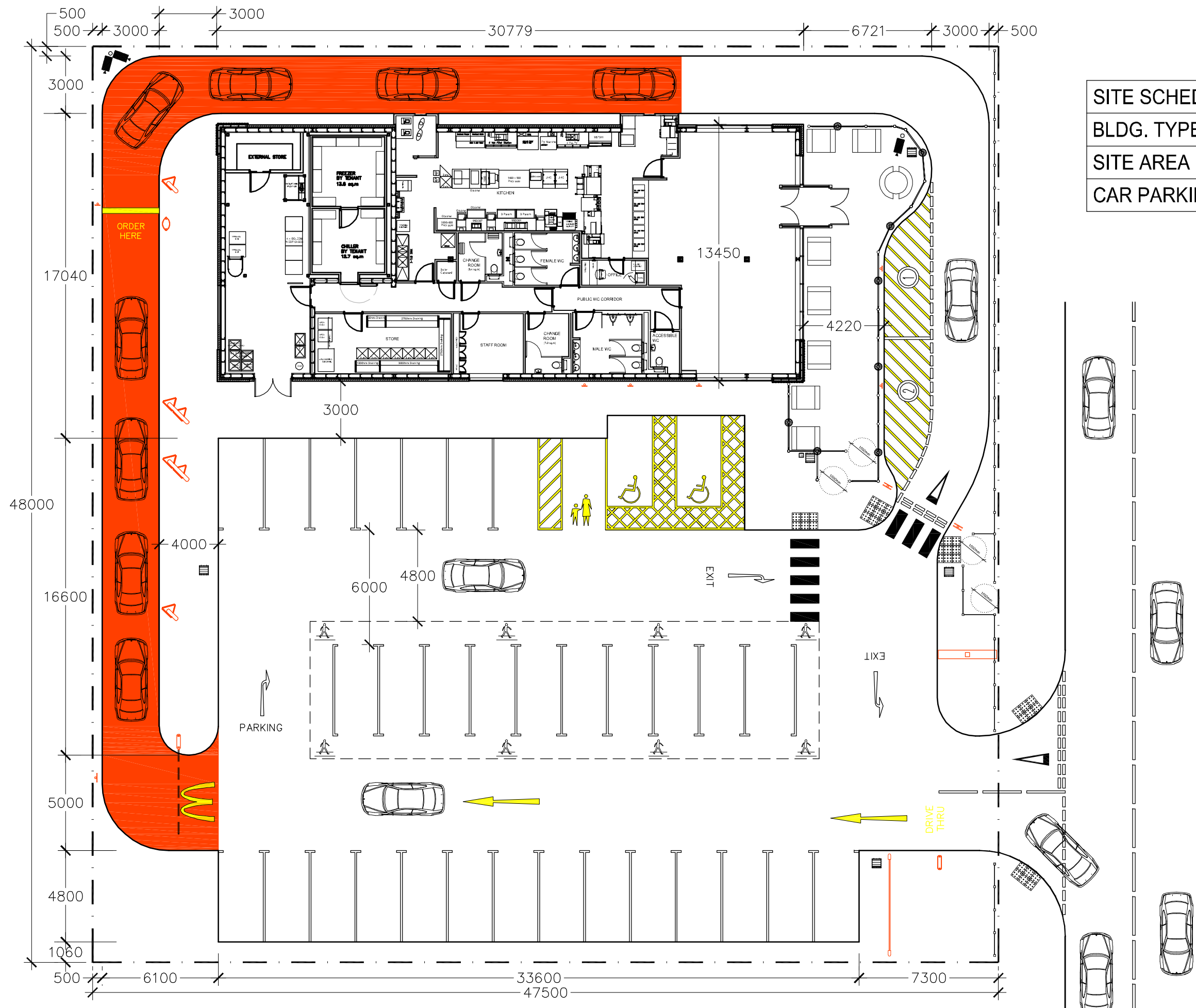
TYPICAL McDONALD'S SITE LAYOUT INCORPORATING AN F60 BUILDING FOOTPRINT
